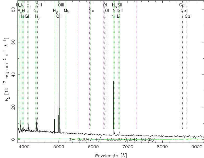
Figure 3: An SDSS spectrum of the galaxy SDSS J13504.5+051122.2 at a redshift of z = 0.0047 . Because it visually appears to be a dwarf irregular and its spectra has a strong H\alpha line, it is likely that HI will be detected.
