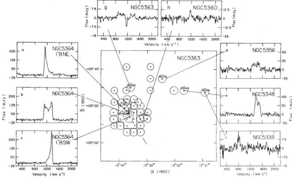
Figure 2: A map of pointings and corresponding spectra from Haynes (1981) of the LGG 362 group. The drift at \delta(J2000) = +05^\circ 13' 54'' will cover NGC 5363, NGC 5356, NGC 5348, and NGC 5338, as well as three other expected detections not shown in this image.
