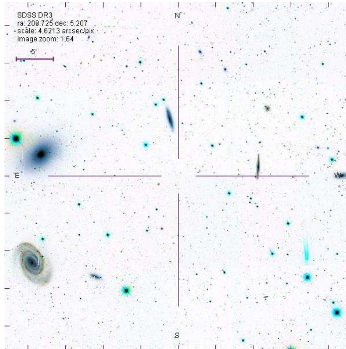
Figure 1: An SDSS image of the LGG 362 group, centered at \alpha(\text{J2000}) = 13^{\text{h}}54^{\text{m}}54^{\text{s}} , \delta = +05^{\circ}12'25'' . NGC 5363 is located in the middle left area of the image, while the four other galaxies in the central strip are expected detections. NGC 5364, the other large galaxy in the group, is located in the lower left corner.
