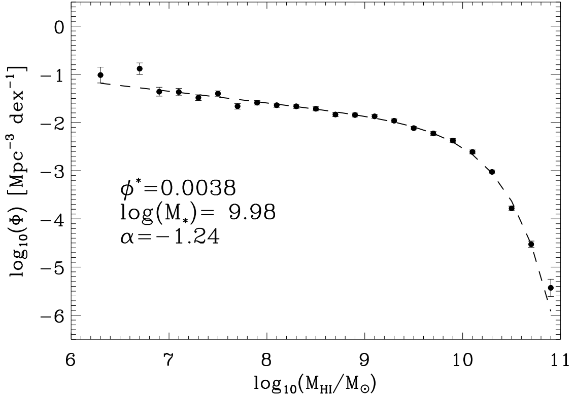
Fig. 18.— The HI mass function obtained via the 2DSWML method when distances, and therefore masses, are obtained assuming pure Hubble flow with H_0 = 70 \text{ km s}^{-1}\text{Mpc}^{-1} . As anticipated by Masters (2005), the adoption of pure Hubble flow yields an underestimate of the low HI mass slope \alpha .
